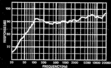
FREQUENCY RESPONSE
